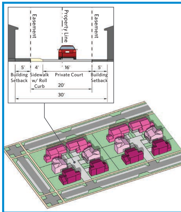
Figure 3.11 Townhouses Private drive cluster homes (small-lot subdivision example)
