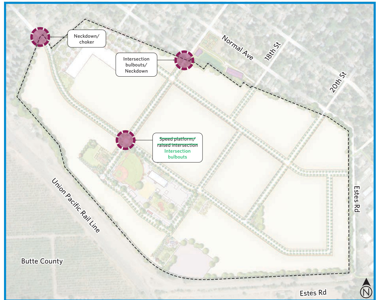
Figure 5.29 Mini-circle Plan of possible likely traffic calming locations
