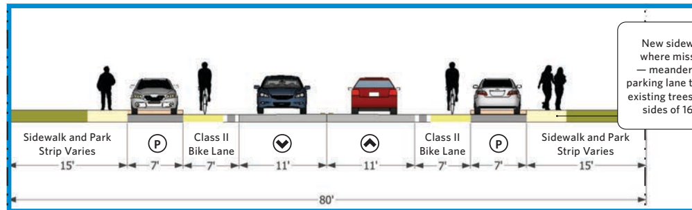
Figure 5.14 16th Street outside of BYSP Area
