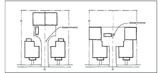
Figure 3.5 Setbacks Shared driveway example
