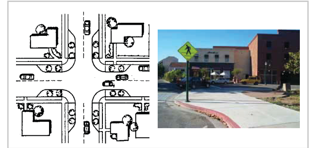
Figure 5.37 Turn restrictions/forced turn island Intersection bulbouts/neckdown
