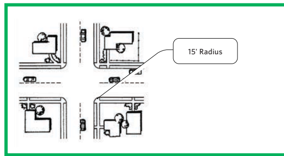
Figure 5.36 Half-closure 15-foot intersection radius at curb returns
