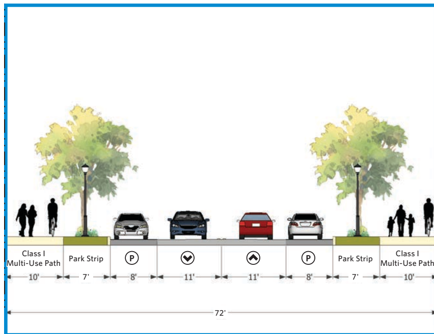
Figure 5.16 Ivy Street within BYSP Area
