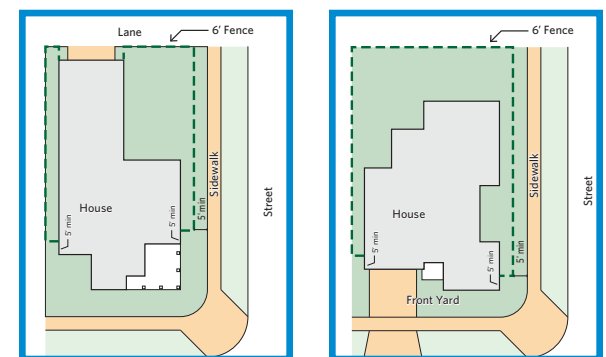
Figure 3.15 Fence requirements plan
