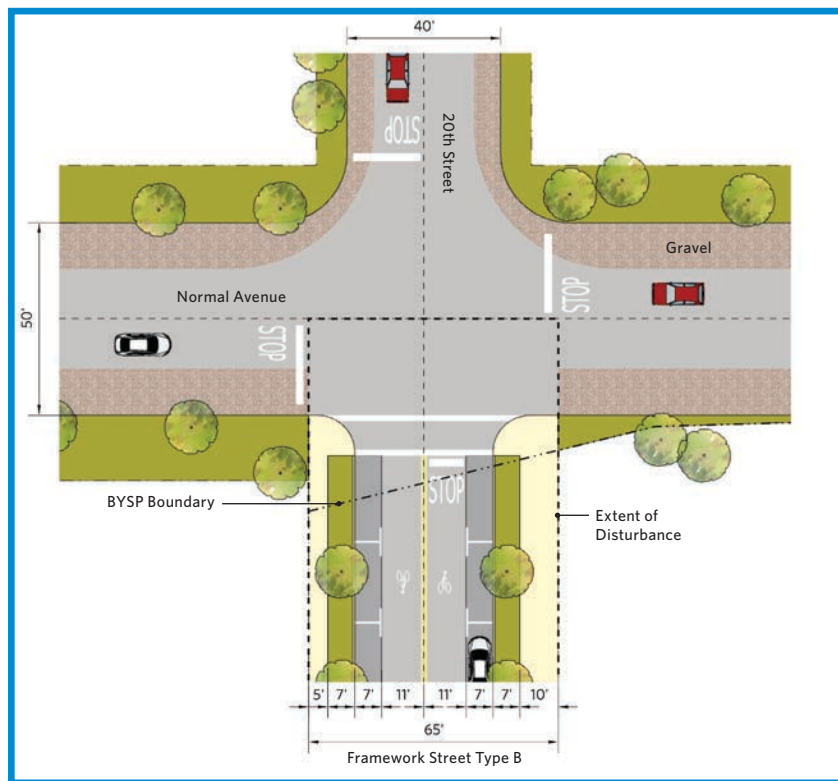
Figure 5.28 C 20th Street Connection
