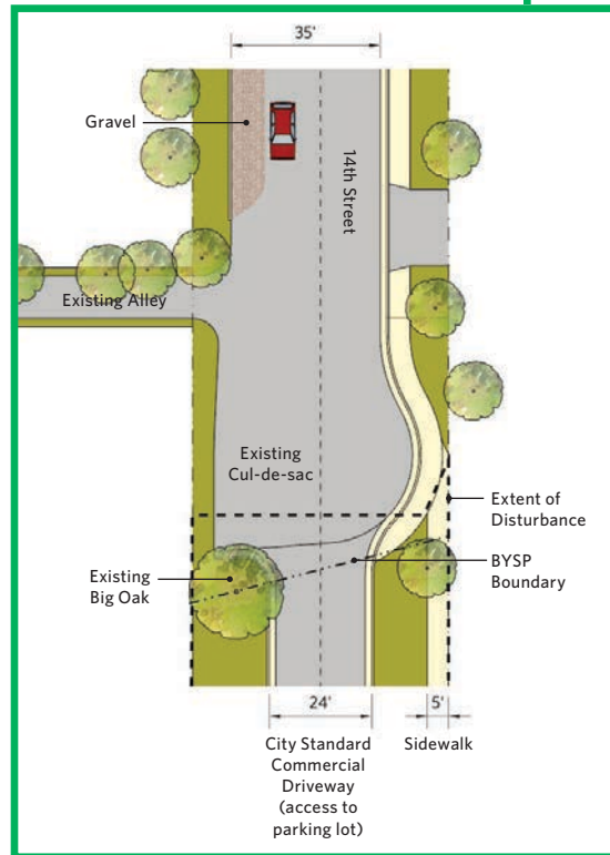
Figure 5.28 A 14th Street Connection
