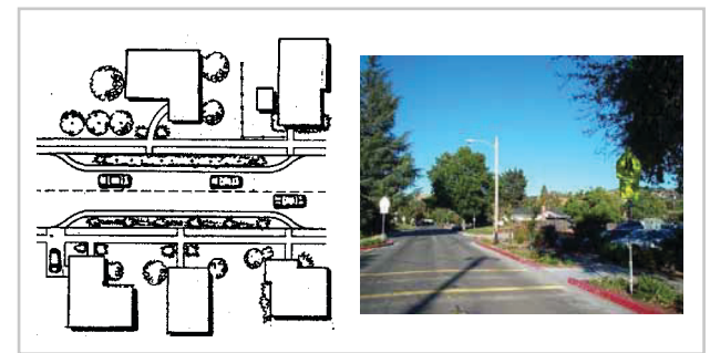
Figure 5.39 Neckdown/choker
