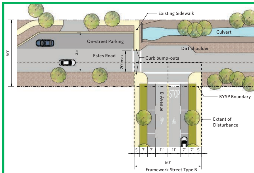
Figure 5.28 D Estes Road Connection
