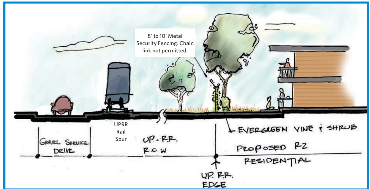
Figure 4.57 Section
