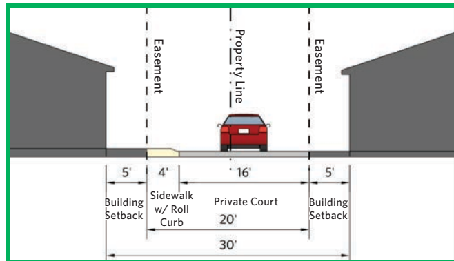
Figure 5.28 Residential Alley Type B (Private) Private Drive (See figure 3.11)
