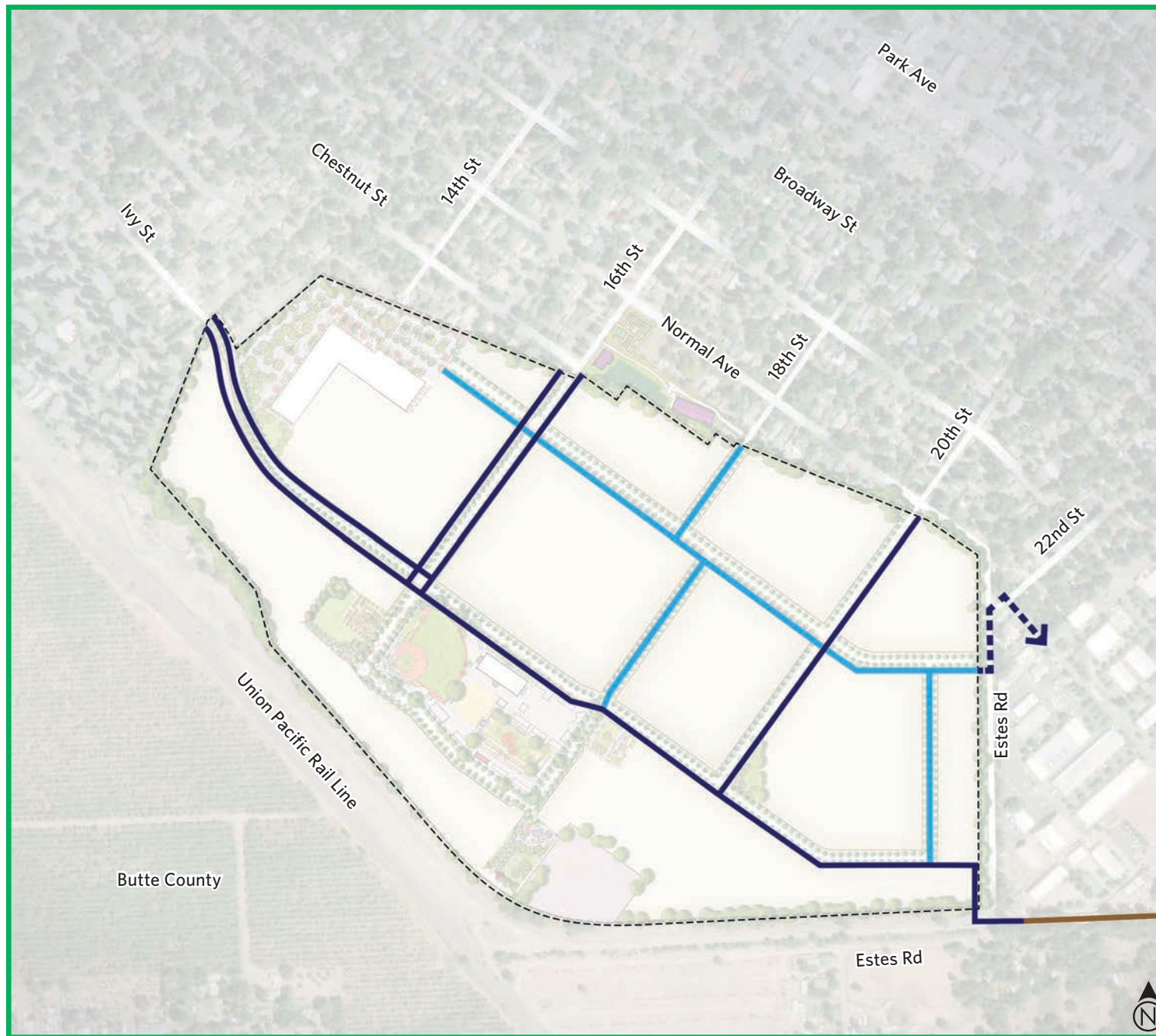
Figure 5.11 Bicycle infrastructure plan
