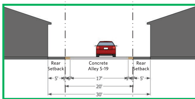
Figure 5.27 Residential Alley Type A (Public)
