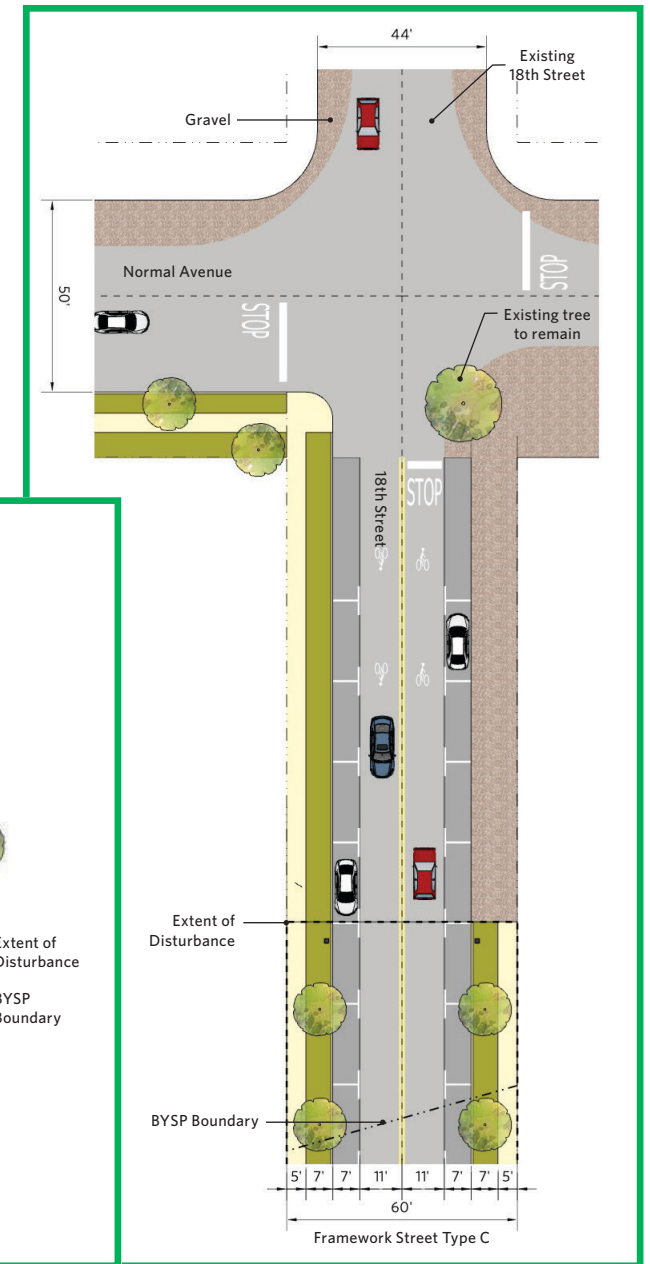
Figure 5.28 B 18th Street Connection
