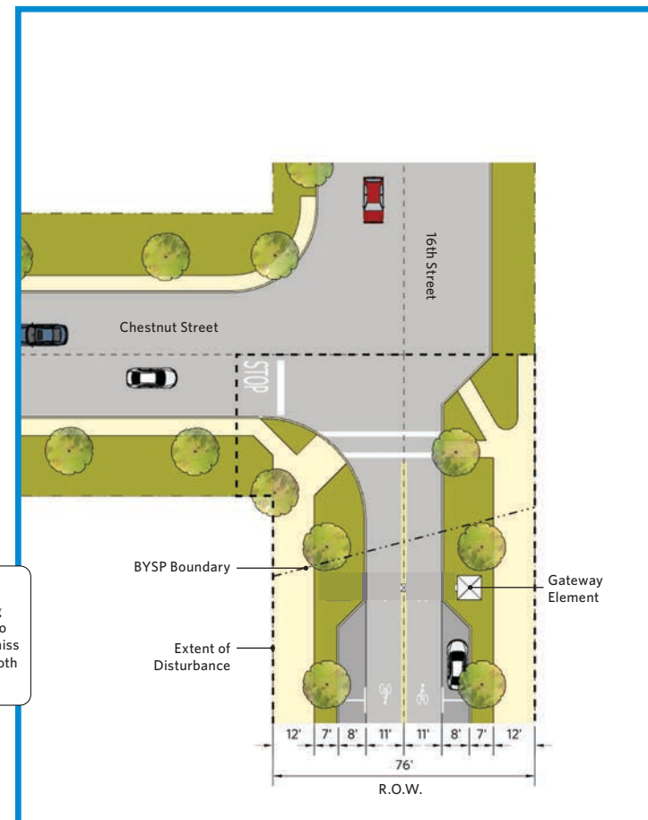
Figure 5.15 Transition area where 16th Street crosses in and out of the BYSP Area
