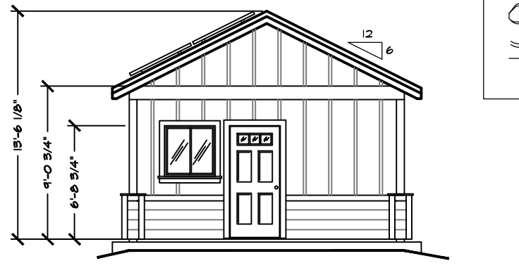
FRONT ELEVATION 1/8" = 1'-0"
