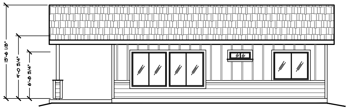
RIGHT ELEVATION 1/8" = 1'-0"
