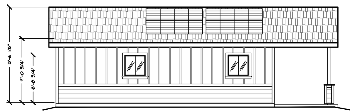
LEFT ELEVATION 1/8" = 1'-0"
