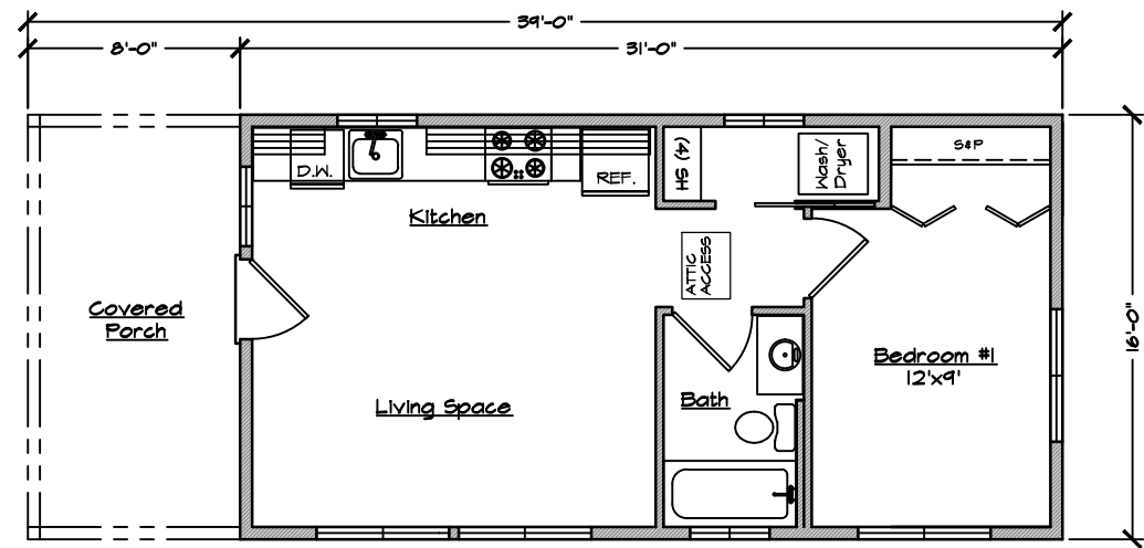
FLOOR PLAN 496 SQ. FT. 1/8" = 1'-0"
