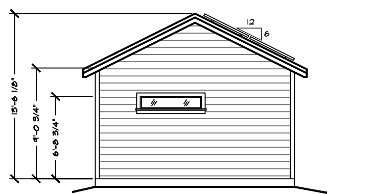
REAR ELEVATION 1/8" = 1'-0"
