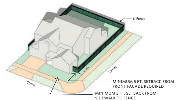
Figure 3.14 Front-loaded lot fence
