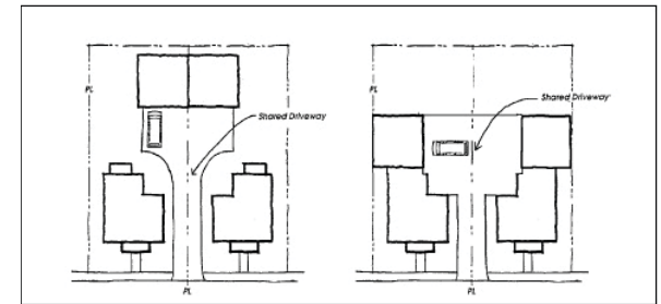
Figure 3.5 Shared driveway example
