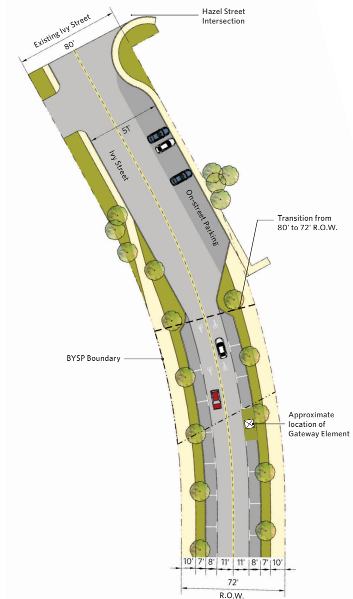
Figure 5.18 Transition area where Ivy Street crosses in and out of the BYSP Area
