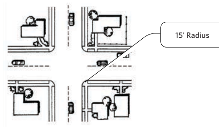
Figure 5.36 15-foot intersection radius at curb returns
