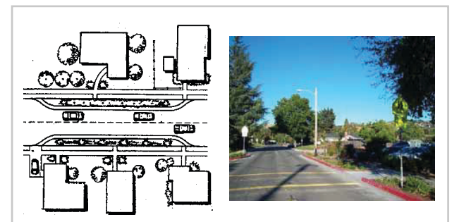
Figure 5.39 Neckdown/choker
