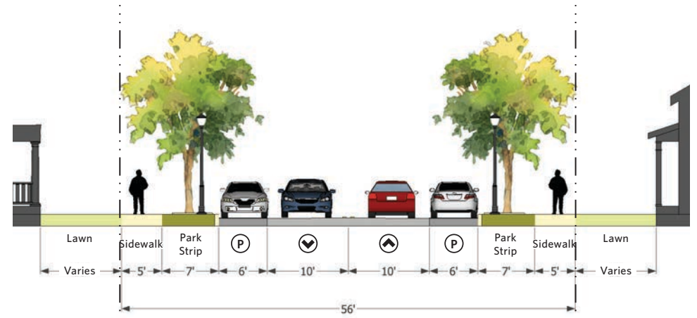
Figure 5.25 Supporting Street Type C
