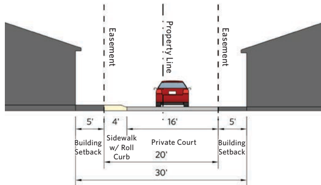
Figure 5.28 Private Drive (See figure 3.11)
