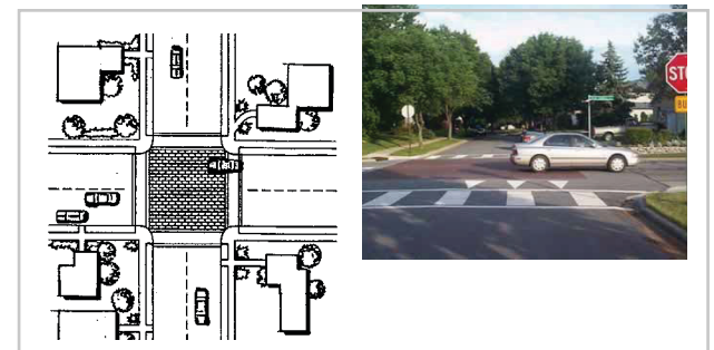
Figure 5.38 Speed platform/raised intersection
