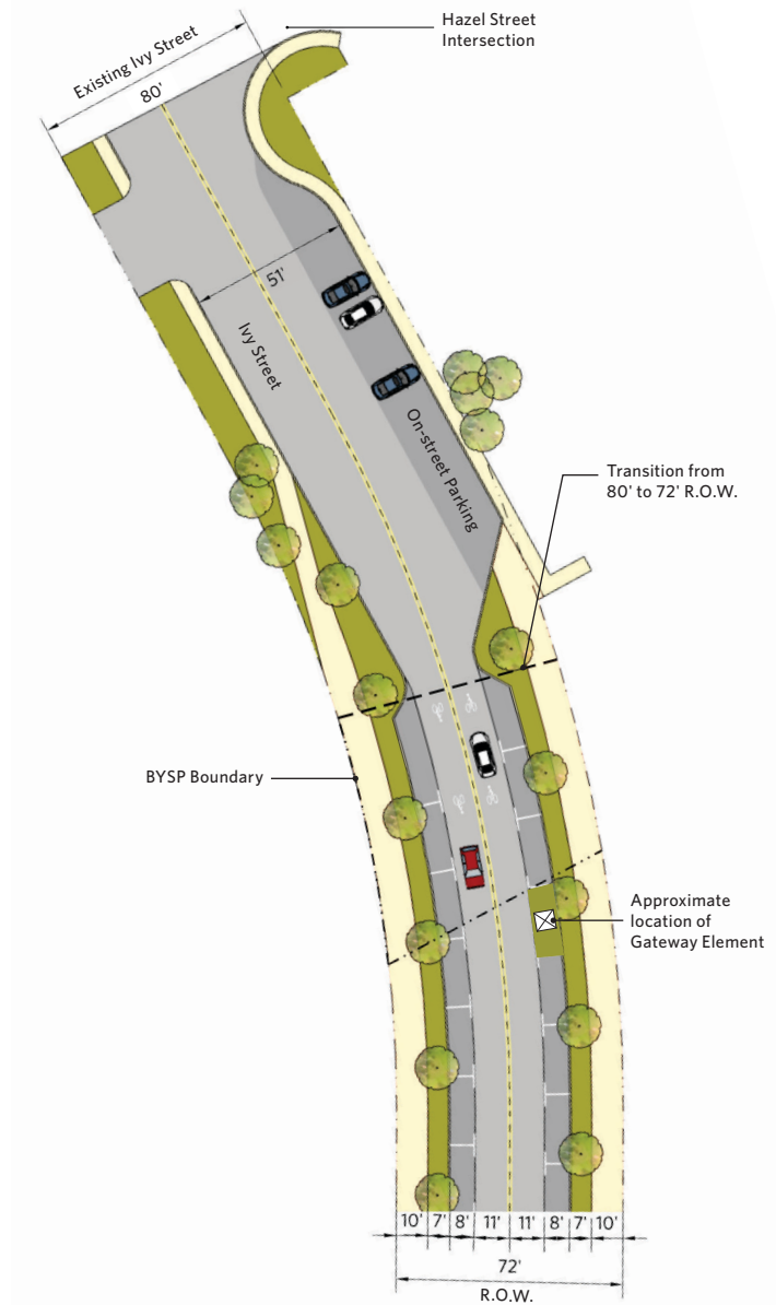
Figure 5.18 Transition area where Ivy Street crosses in and out of the BYSP Area
