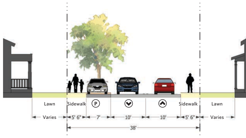
Figure 5.24 Supporting Street Type B
