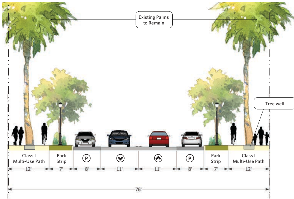
Figure 5.13 16th Street within BYSP Area
