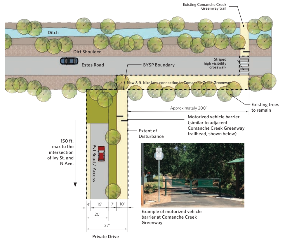
Figure 5.28 E Public Bike Path Connection
