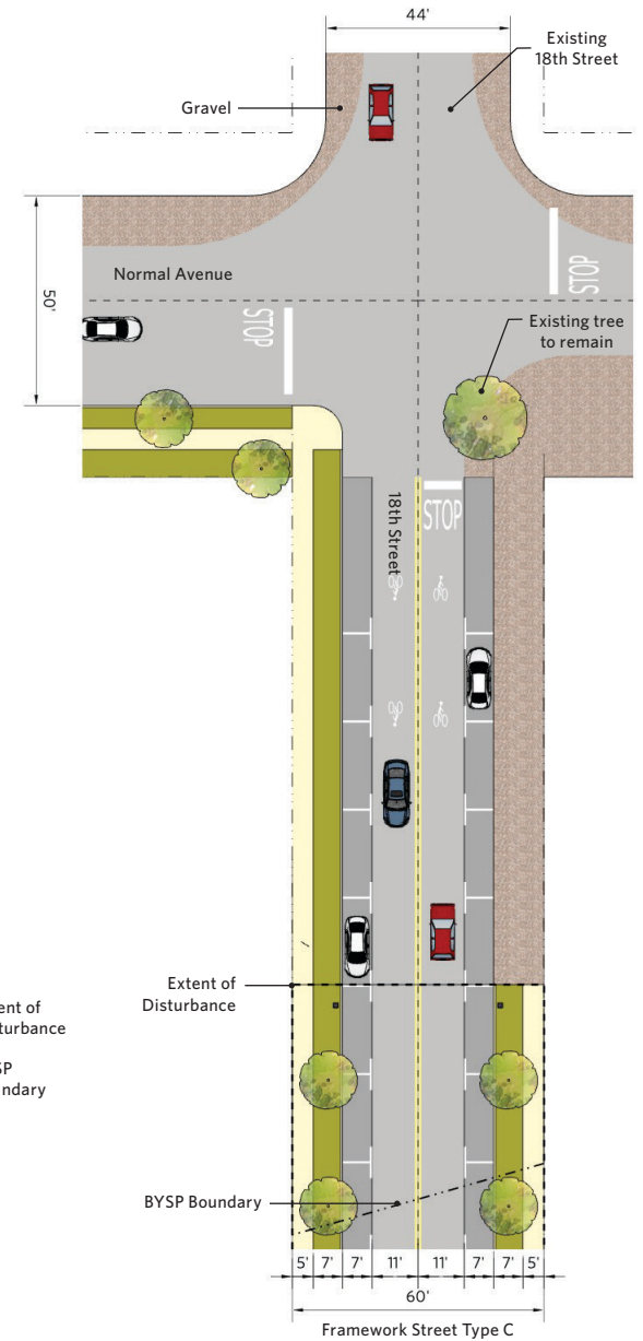
Figure 5.28 B 18th Street Connection
