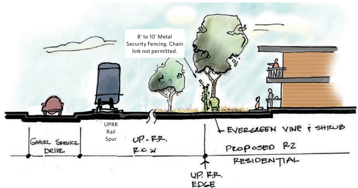
Figure 4.57 Section
