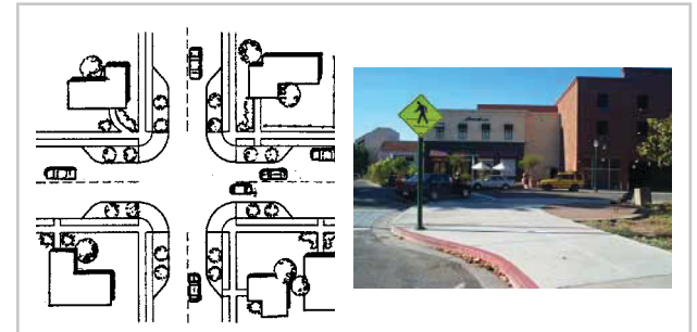
Figure 5.37 Intersection bulbouts/neckdown
