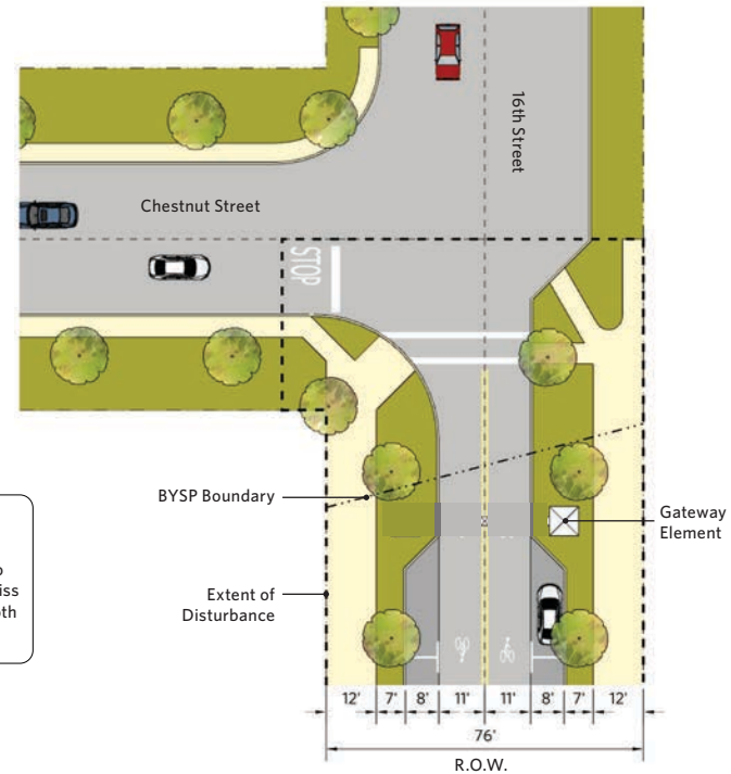
Figure 5.15 Transition area where 16th Street crosses in and out of the BYSP Area
