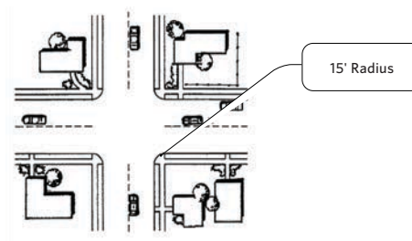
Figure 5.36 15-foot intersection radius at curb returns
