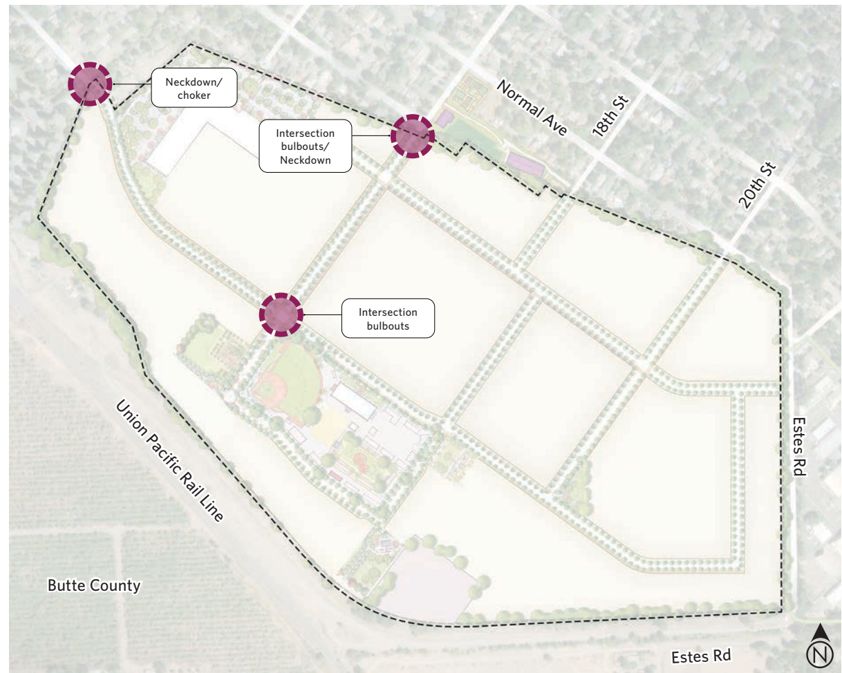
Figure 5.29 Plan of likely traffic calming locations
