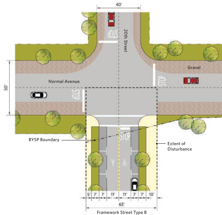
Figure 5.28 C 20th Street Connection
