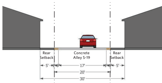
Figure 5.27 Residential Alley (Public)
