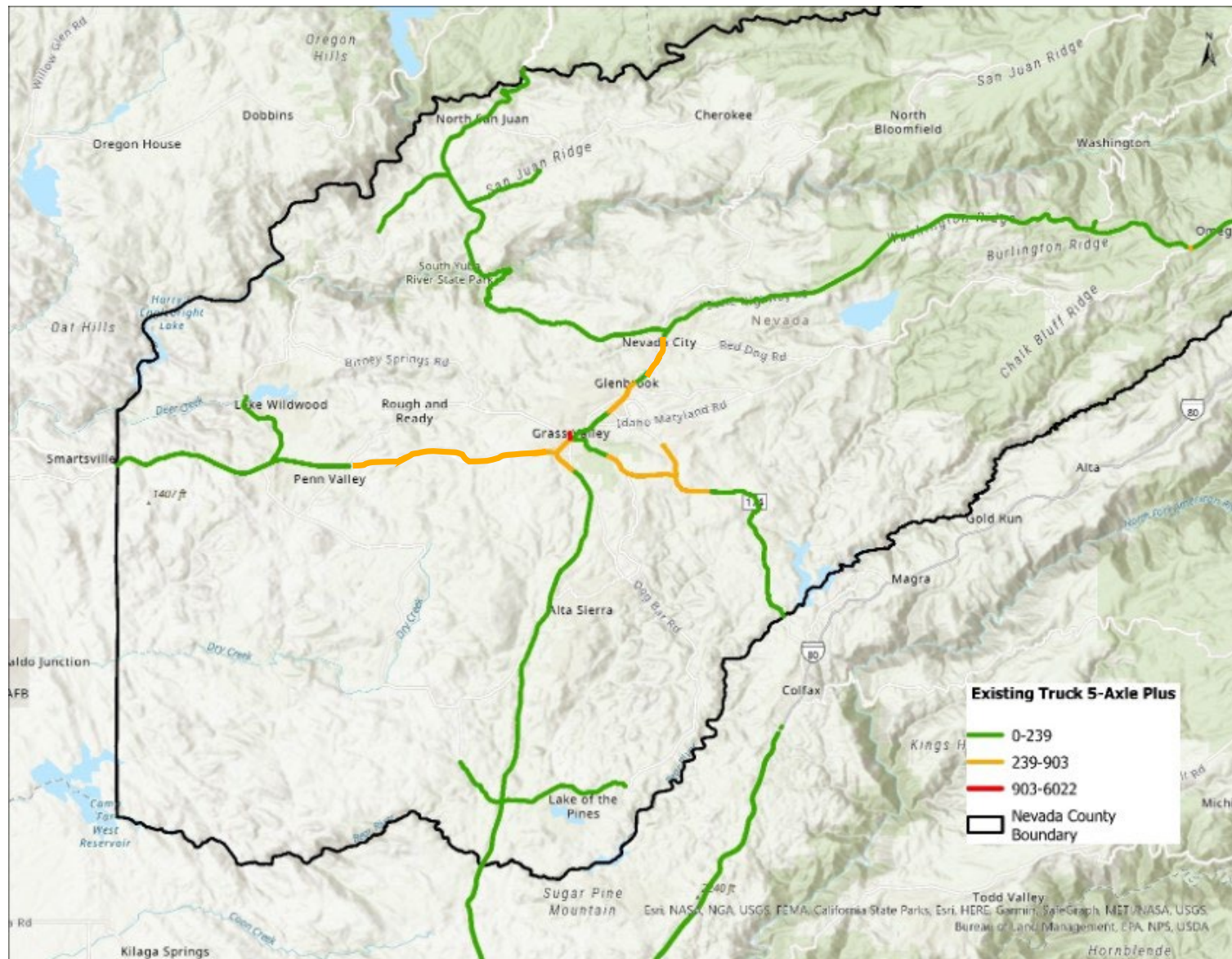
FIGURE 38: EXISTING 5-AXLE OR MORE AADTT
